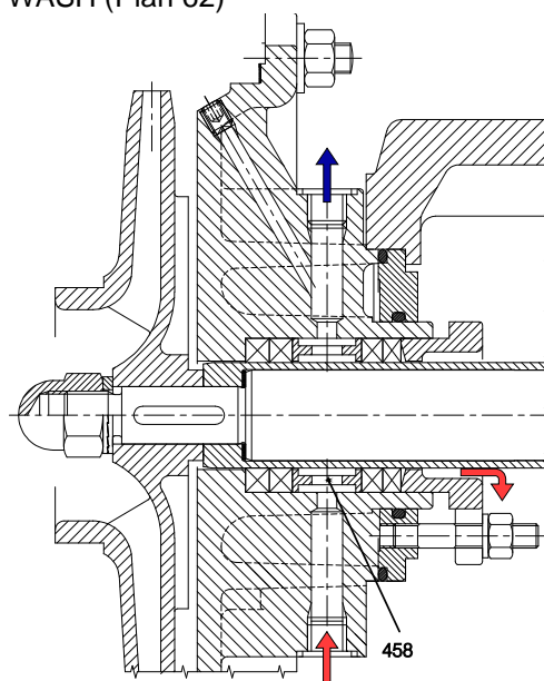
Fig.27d – PACKING WITH EXTERNAL FLUSHING AND WASH (Plan 62)
